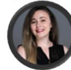
Randa MEZRAG
